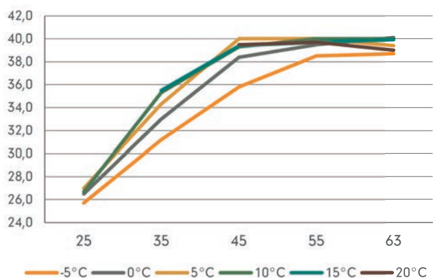
Max. externer Druckverlust, Sole [kPa - l/s]
