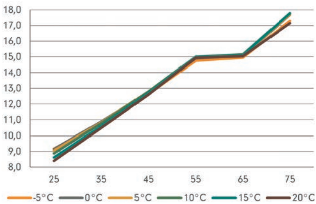
Max. externer Druckverlust, Sole [kPa - l/s]
