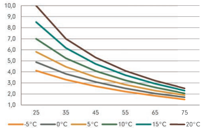
Max. externer Druckverlust, Ladung [kPa - l/s]
