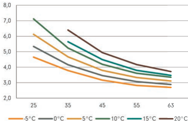
Max. externer Druckverlust, Ladung [kPa - l/s]
